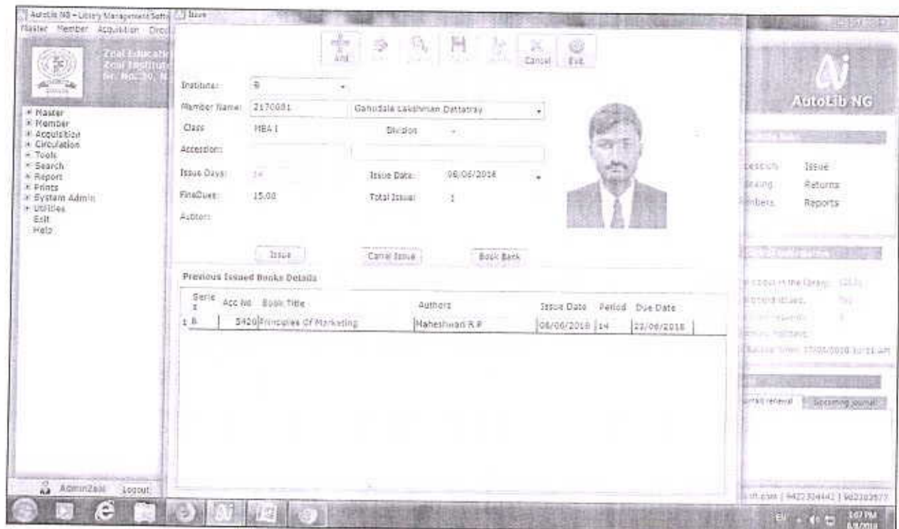
Photo 3. Issue Return
